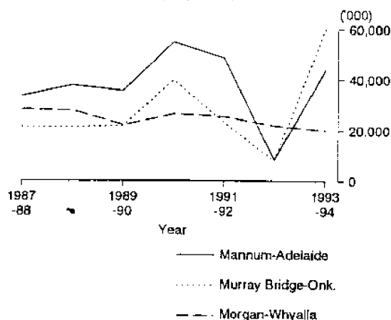
MAIN PIPELINES : WATER PUMPED FROM RIVER MURRAY (Megalitres)
